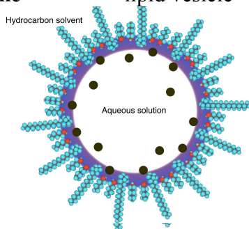
water-in-oil microemulsion
