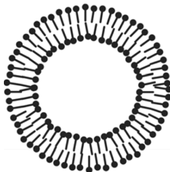
lipid vesicle
